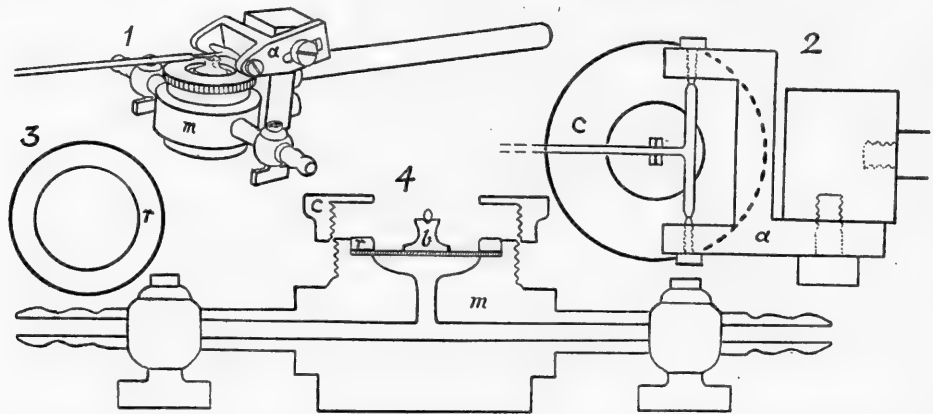
TEST-FIG. 25. Simple form of membrane manometer. —1, small-scale view ; 2, plan from above ; 3, brass ring-washer ; 4, elevation section. 2, 3, and 4 are actual scale. a , slotted adjustable piece carrying the pivot-bearings ; m , the body containing the chamber and tube-borings ; r , the ring-washer fixing the rubber disk-membrane when c , the cover-nut, is screwed down ; b , aluminium button scotined to top surface of the rubber membrane ; the light grass-stem writing-lever rides in a notch cut in the ridge of the button-top.
